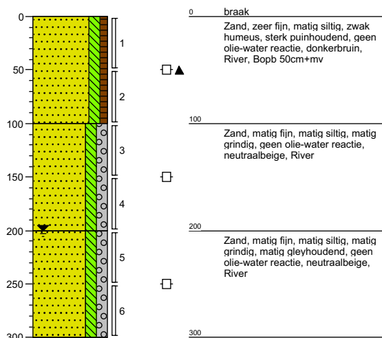
Boring: C02
