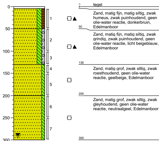
Boring: B03
