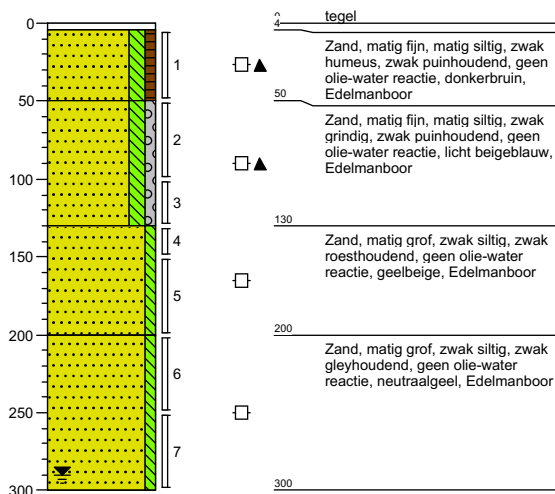
Boring: B02
