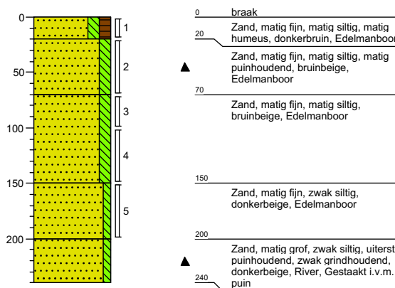
Boring: C01
