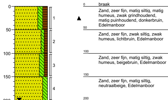
Boring: N01
