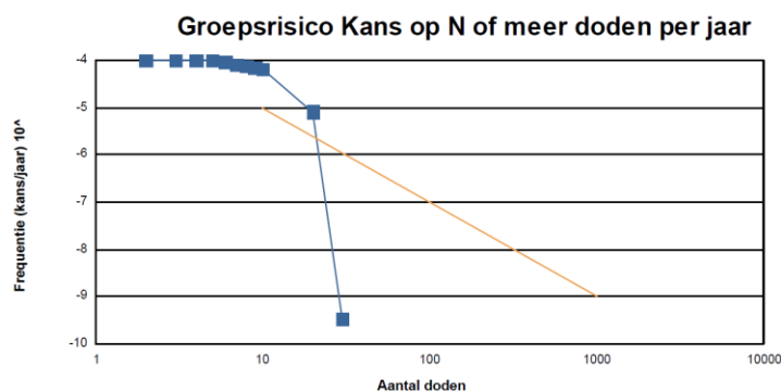
Figuur 4: FN-curve Nouryon Chemicals B.V.
