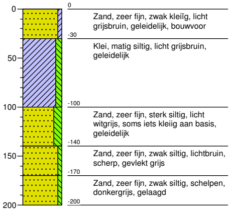
Boring: 26
