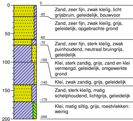
Boring: 3
