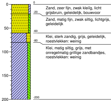
Boring: 7
