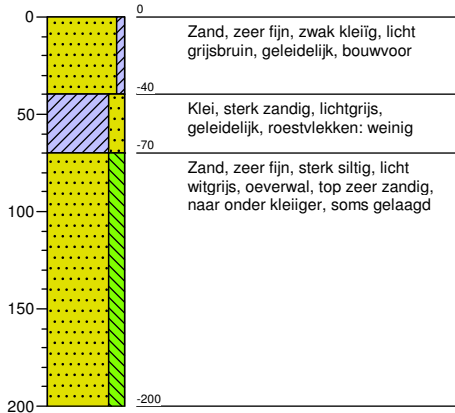
Boring: 11
