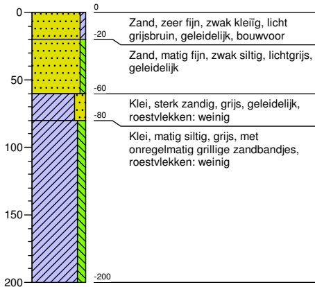
Boring: 8
