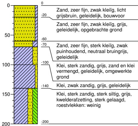
Boring: 4
