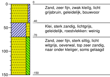
Boring: 12
