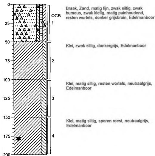
Boring: 5
