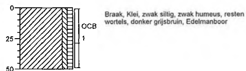
Boring: 7
