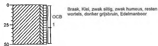
Boring: 12
