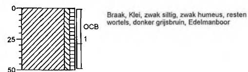
Boring: 13
