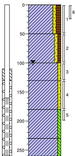
Boring: 01
