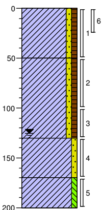
Boring: 02
