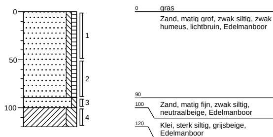
Boring:
