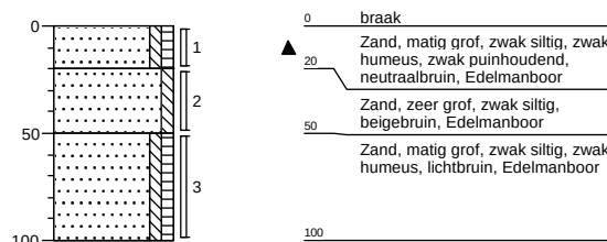
Boring:
