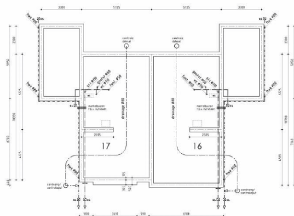
Fundering/Riolering
