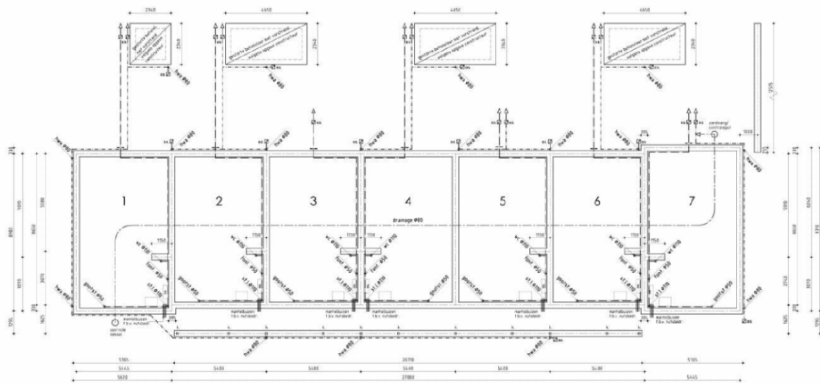
Fundering/Riolering
