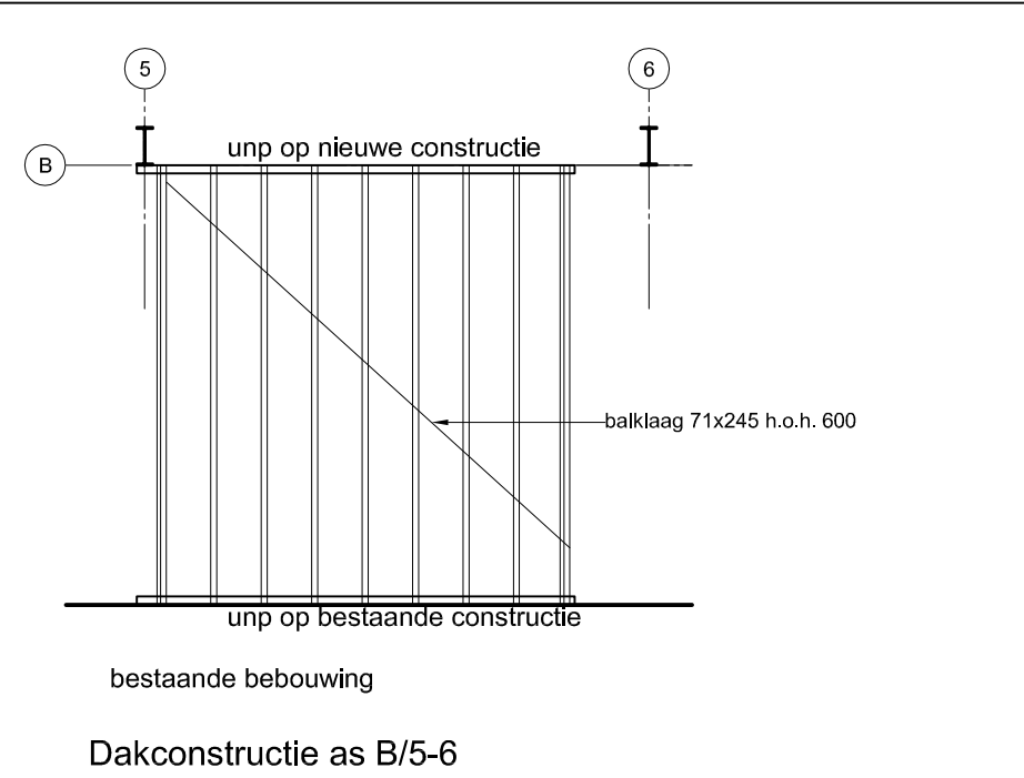
Dakconstructie as B/5-6
