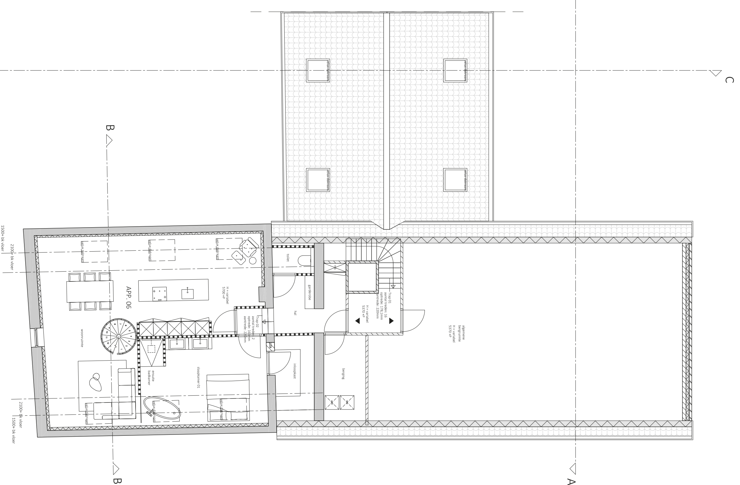
ZOLDER
