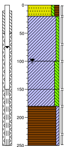
Boring: 08
