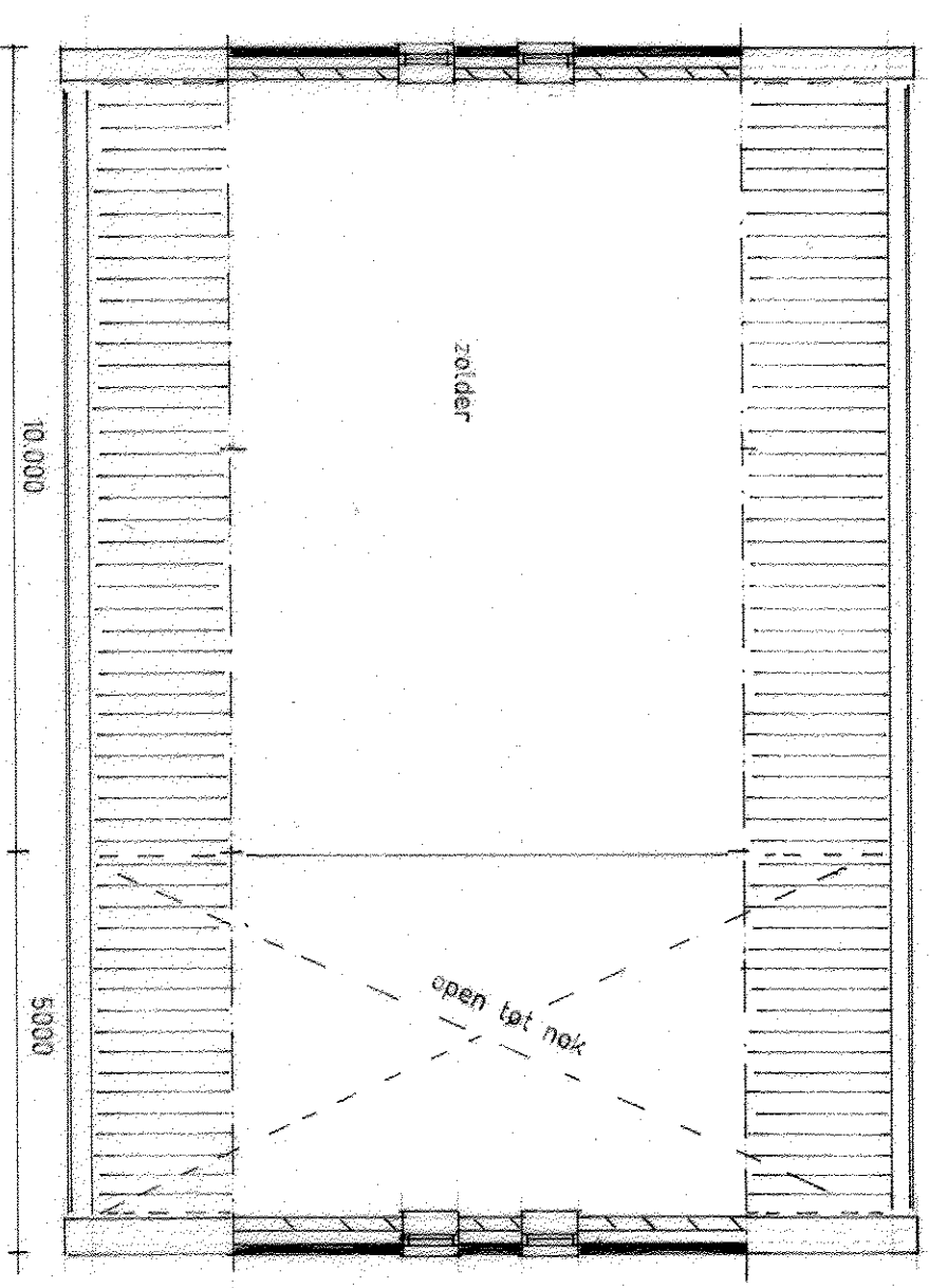
ZOLDER
