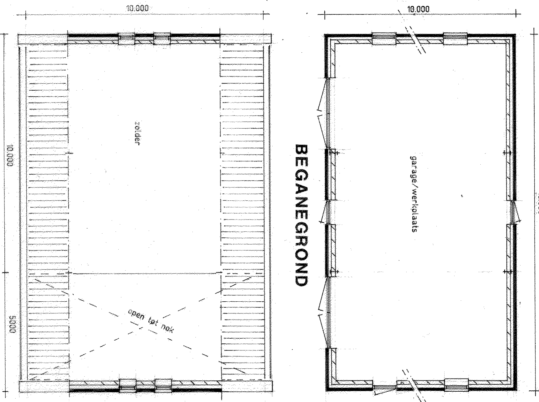
ZOLDER
