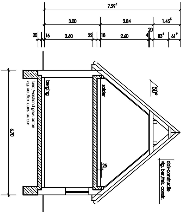
DOORSNED E-B-B
