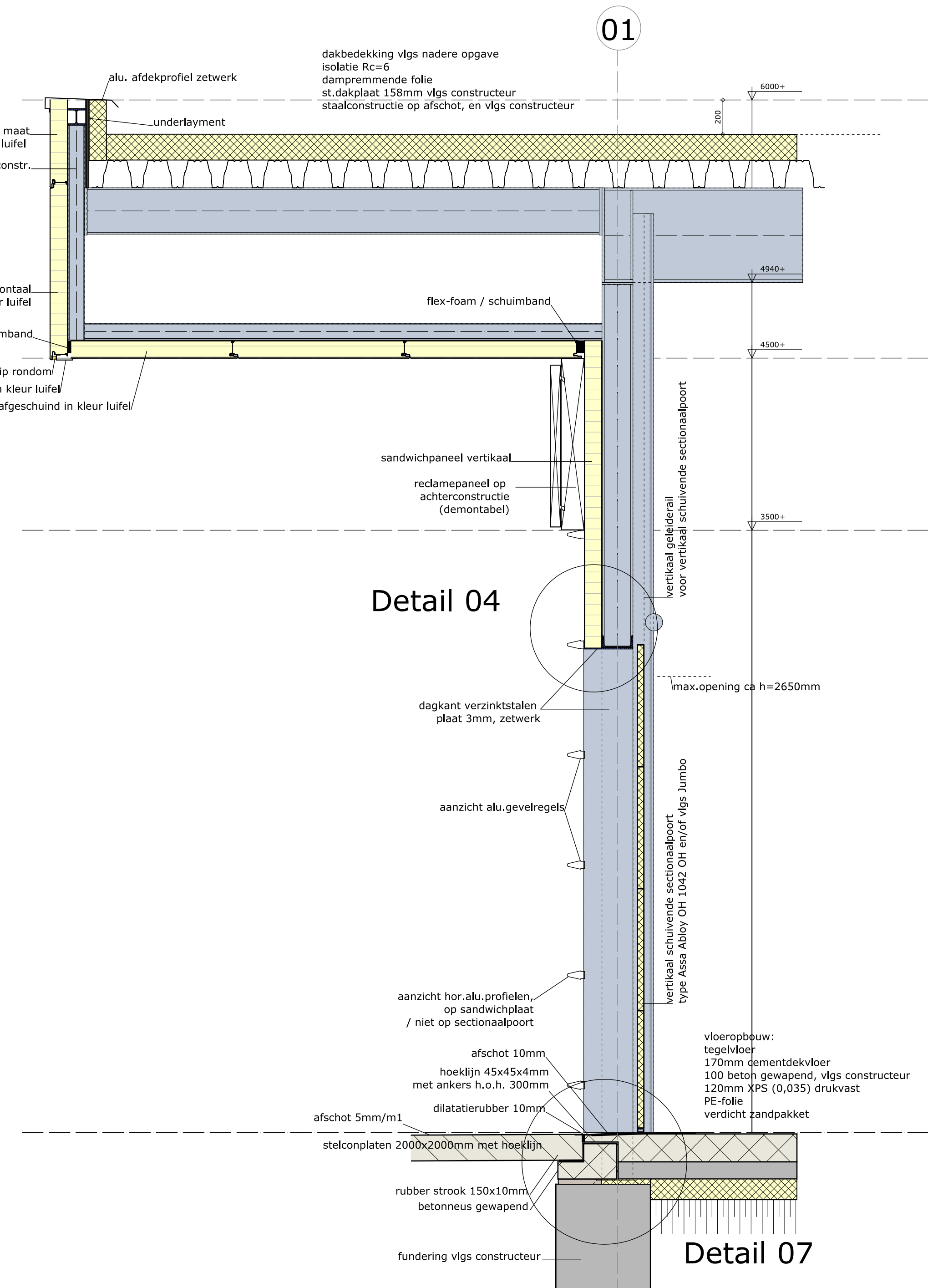
gevelprofiel P03 gevel as 1
