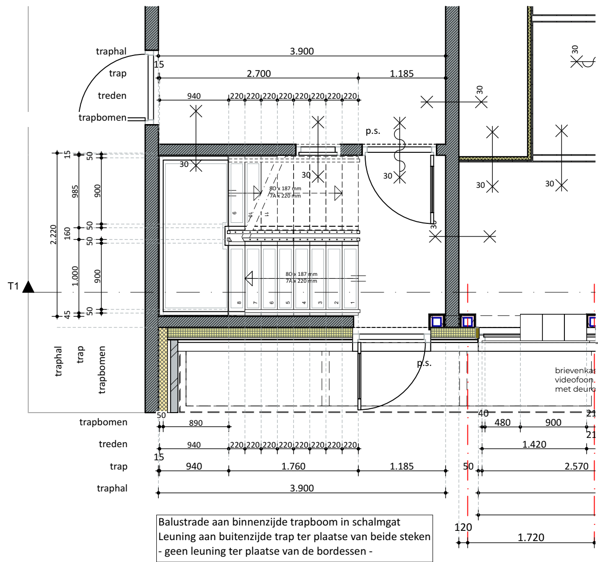
0. Begane grond - Trap 1:50
