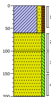
Boring: A06
