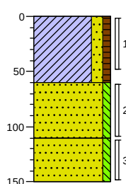
Boring: A02
