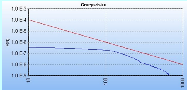
Figuur 2.1 fN-curve
