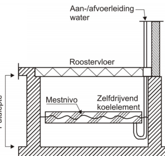
Detail stalsysteem BWL 2010.16.V1 & BWL 2010.17.V1
