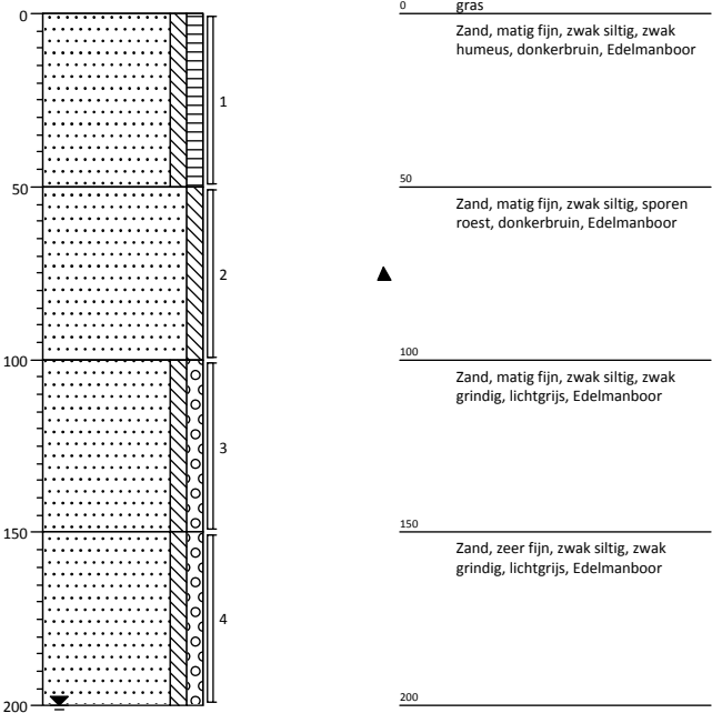
Boring: 02
