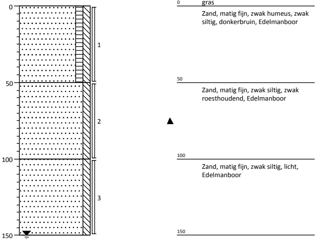
Boring: 02
