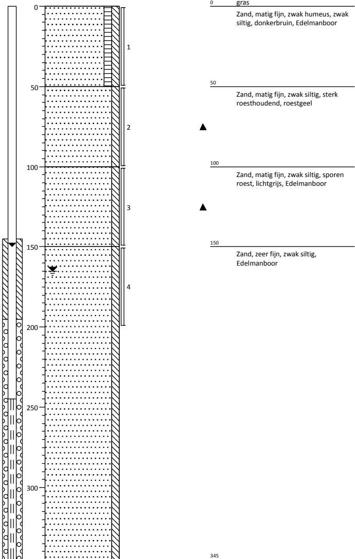
Boring: 01
