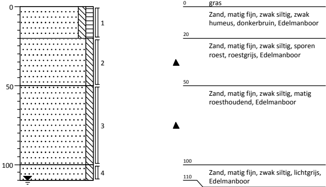
Boring: 04
