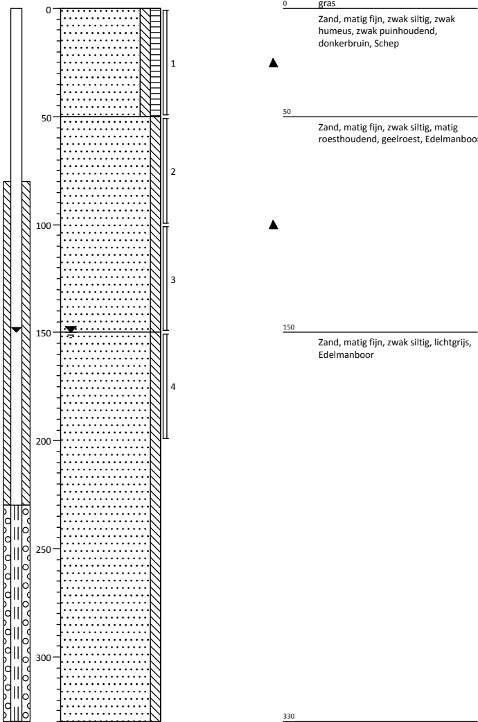
Boring: 01
