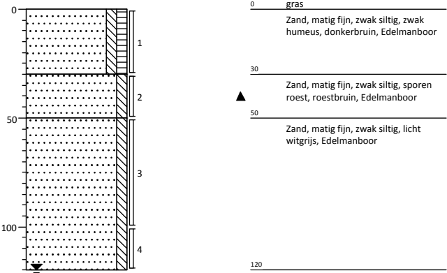
Boring: 03
