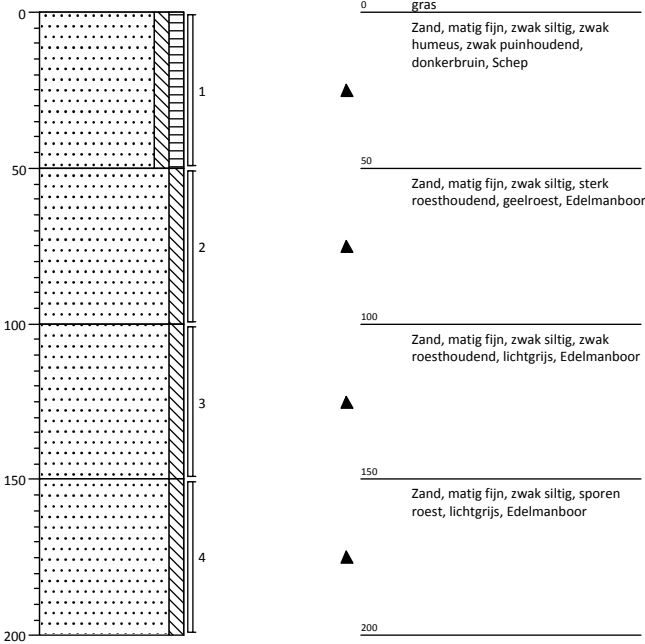
Boring: 02
