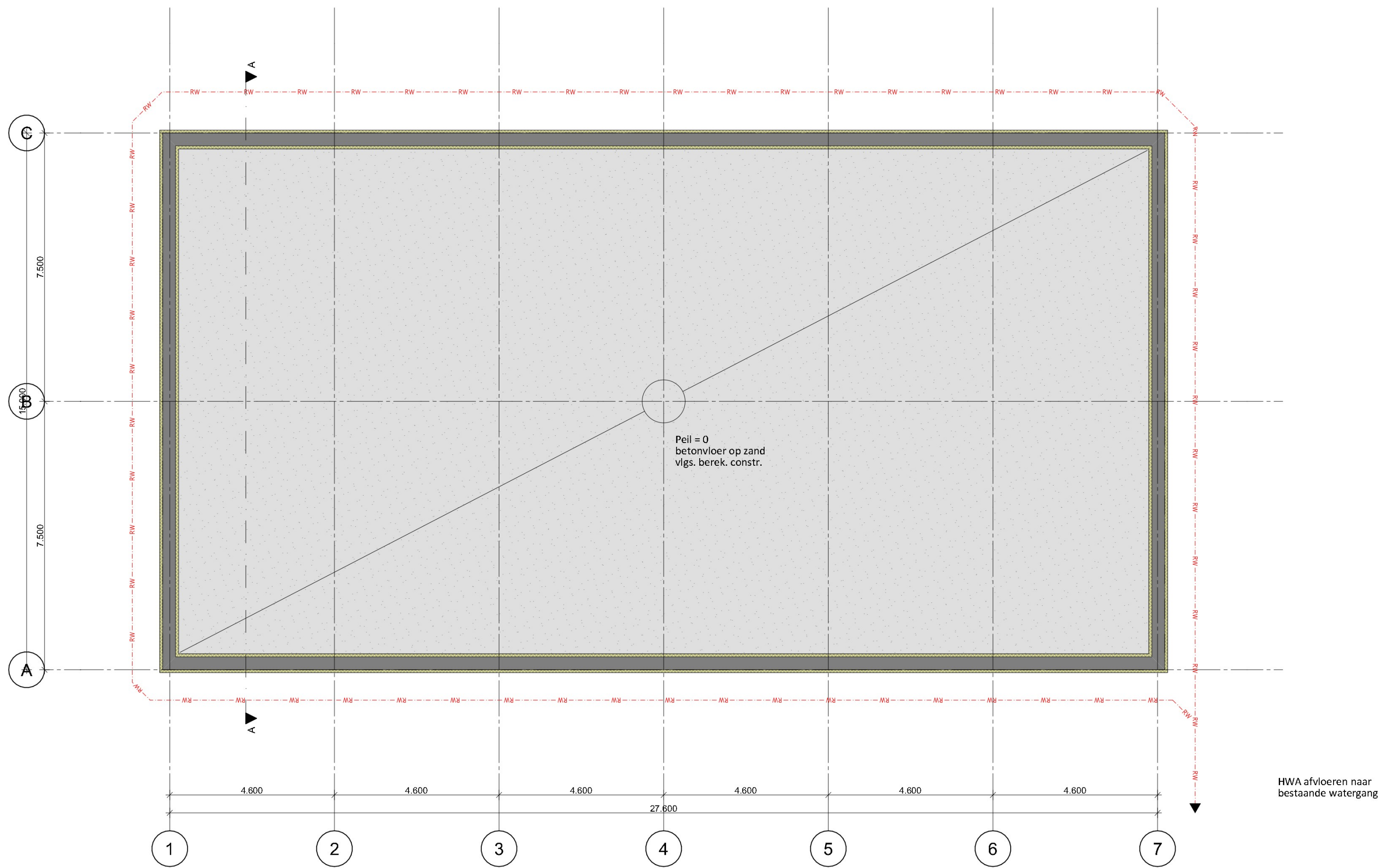
Fundering-rioleringsplan
