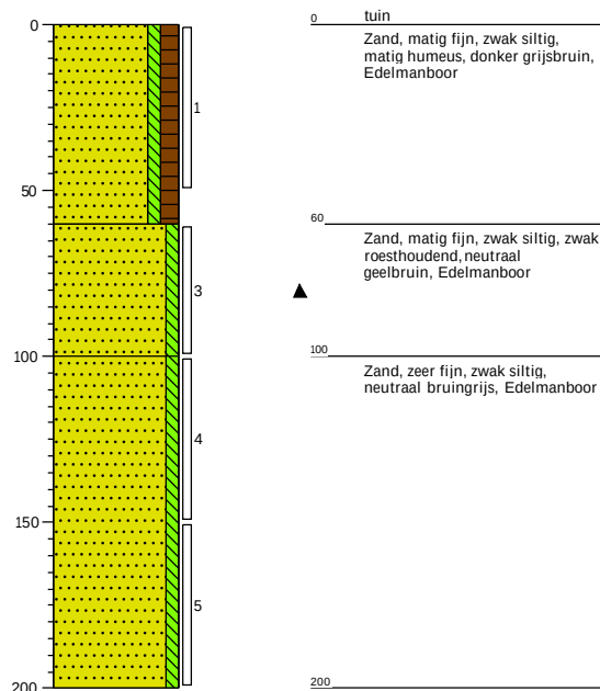
Boring: 10
