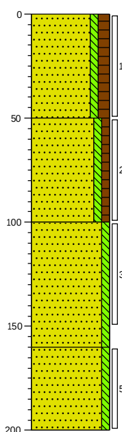
Boring: 03
