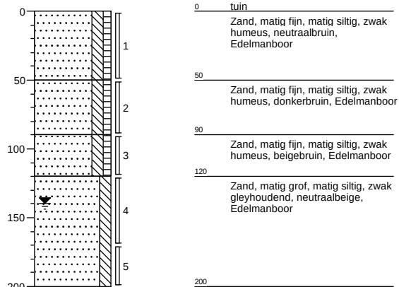
Boring: 02
