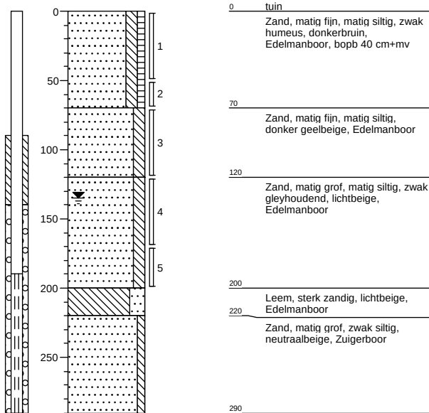
Boring: 01
