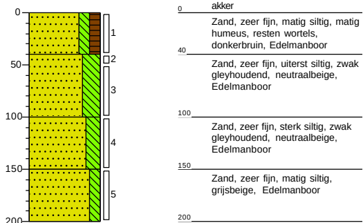
Boring: 03
