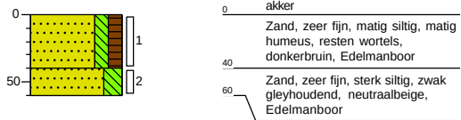
Boring: 05
