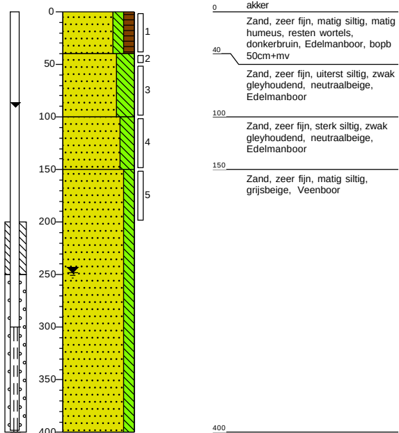
Boring: 01
