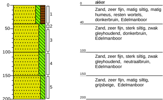
Boring: 02
