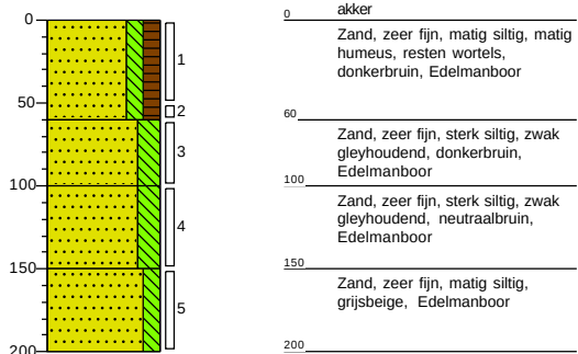
Boring: 04
