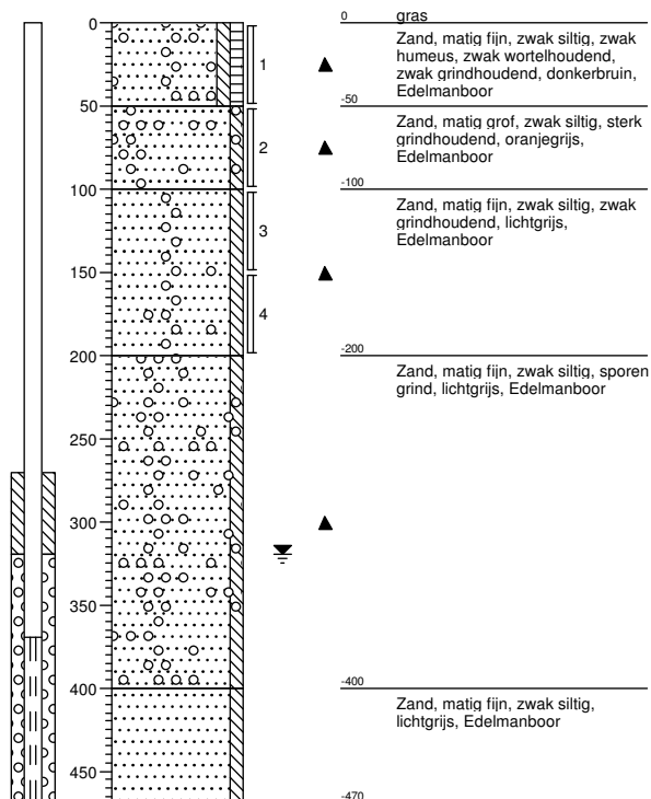
Boring: 1
