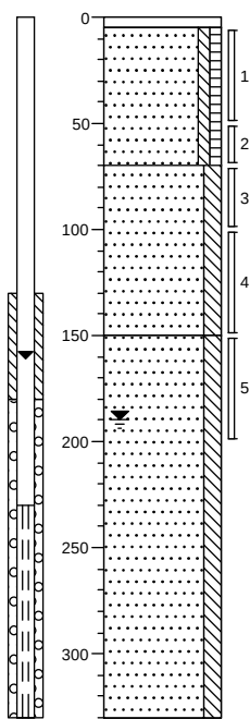
Boring: 01
