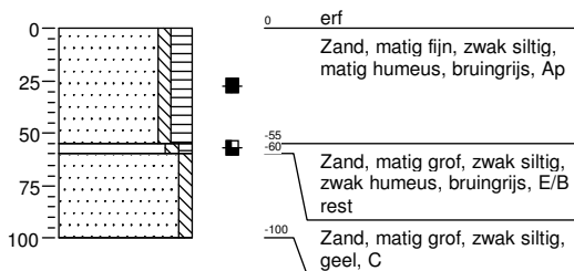
Boring: 044
