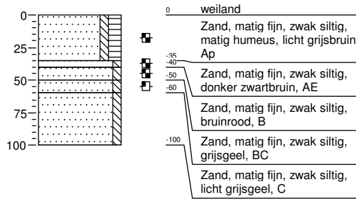
Boring: 008
