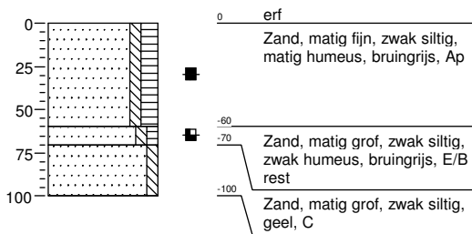
Boring: 043
