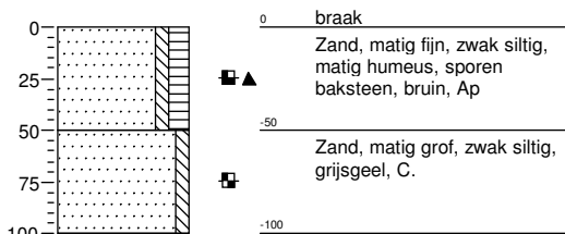
Boring: 038
