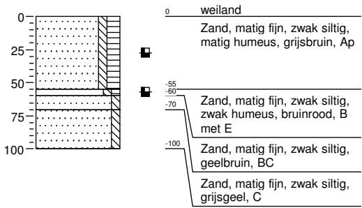
Boring: 011
