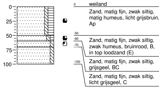
Boring: 009
