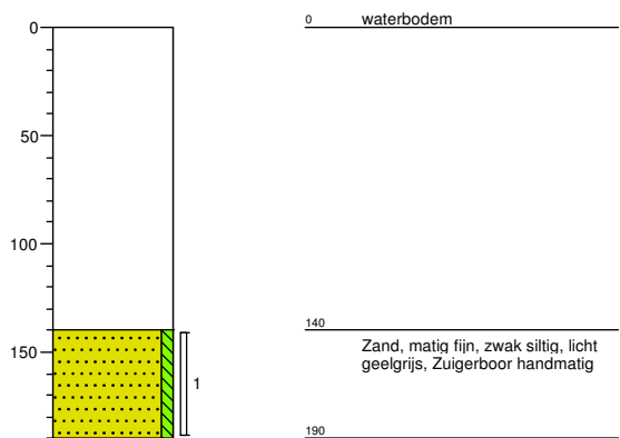
Boring: B03
