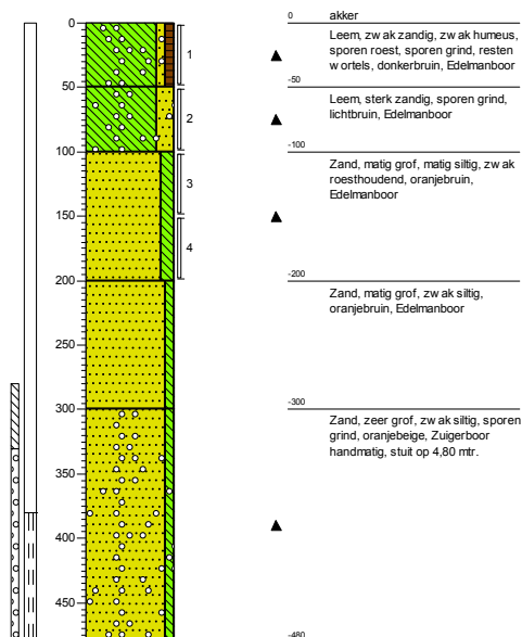
Boring: 15
