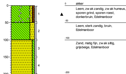
Boring: 13
