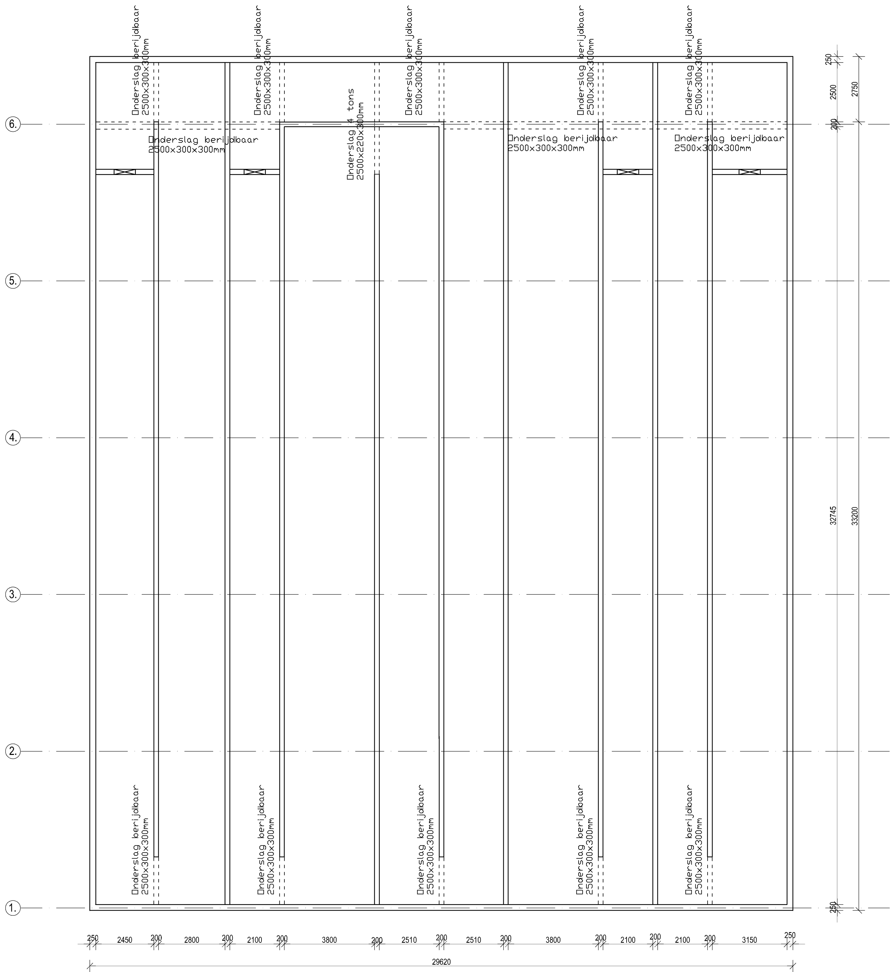
FUNDERINGSPLAN
