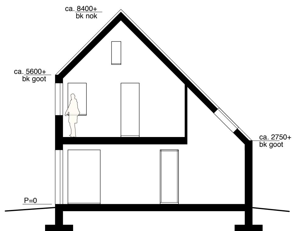
principe dwarsdoorsnede 1a100
