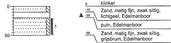
boring 4
