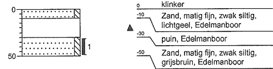
boring 6
