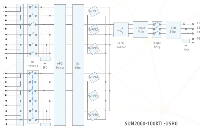
Circuit Diagram
