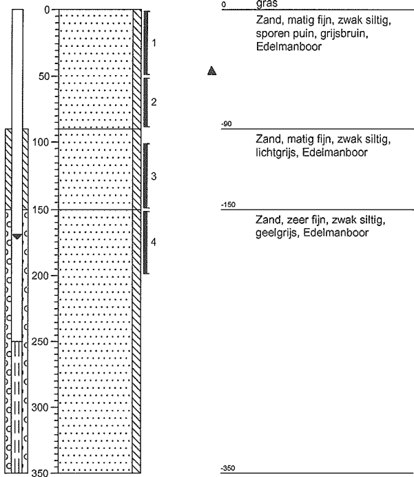
boring 1
