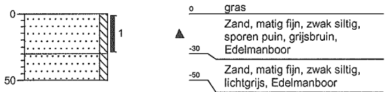
boring 6
