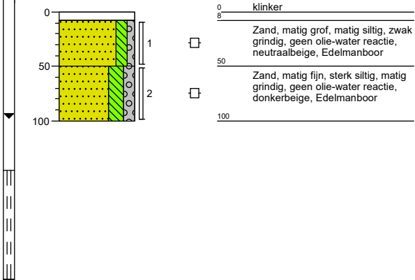
Boring: C02
