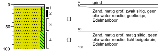
Boring: B01a
