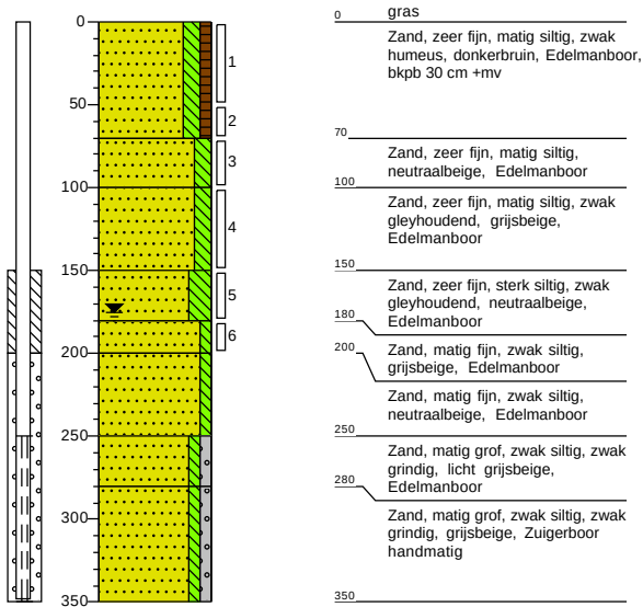
Boring: 01
