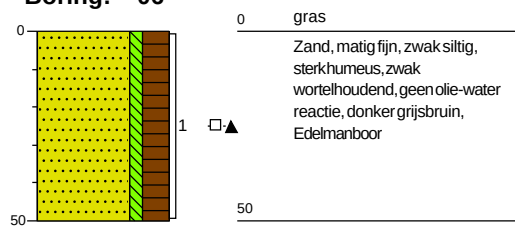
Boring: 06
