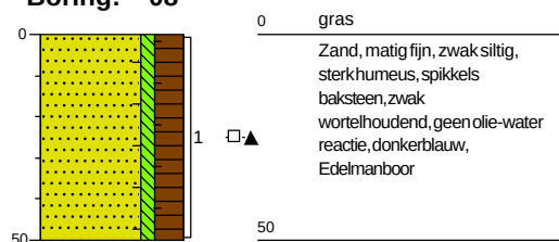
Boring: 08
