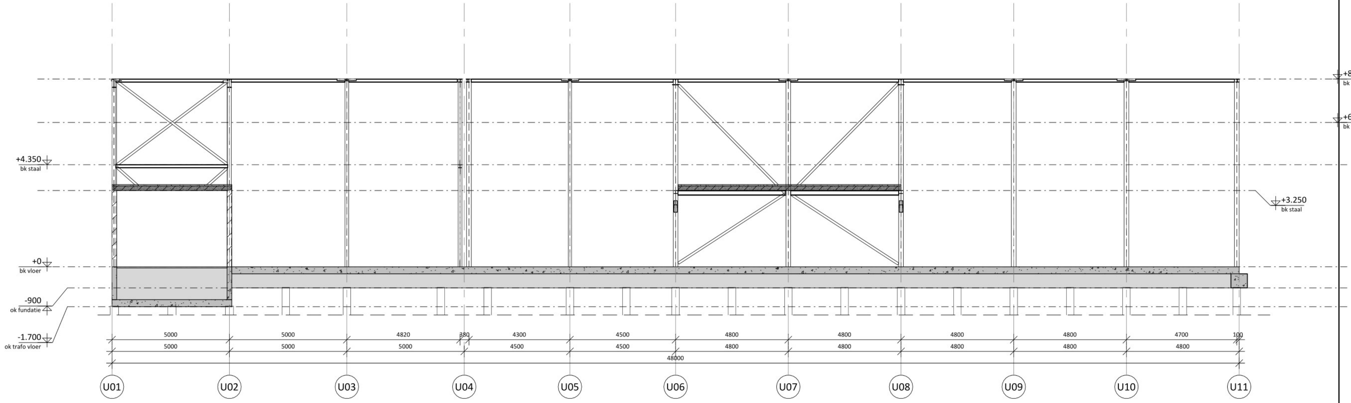
Doorsnede as UG Schaal: 1 : 100
