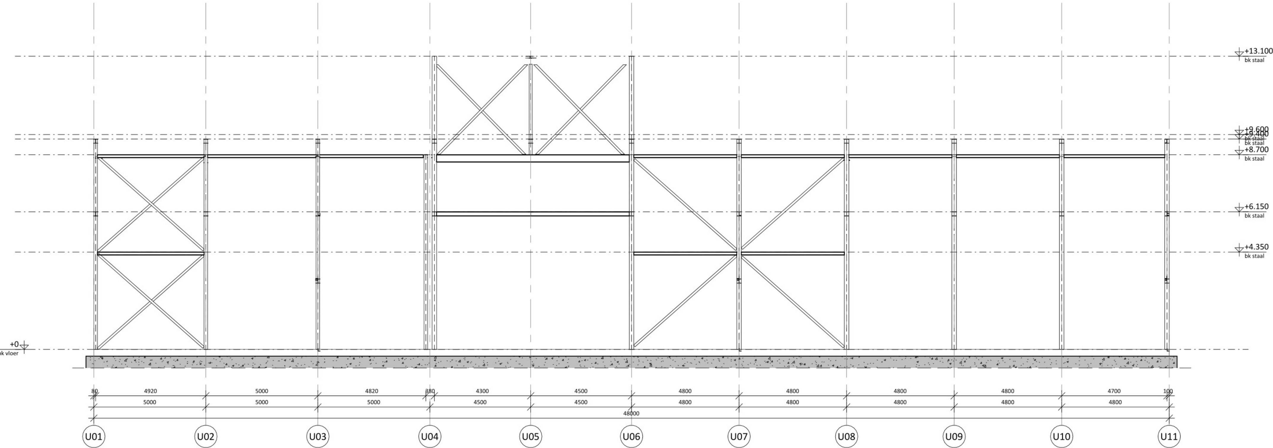
Doorsnede as UA Schaal: 1 : 100
