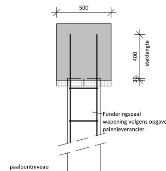
Principe detail poer Schaal: 1:20
