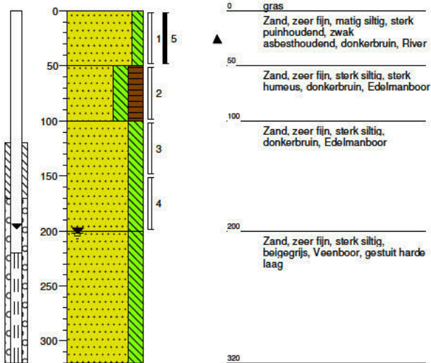
Boring: 01
