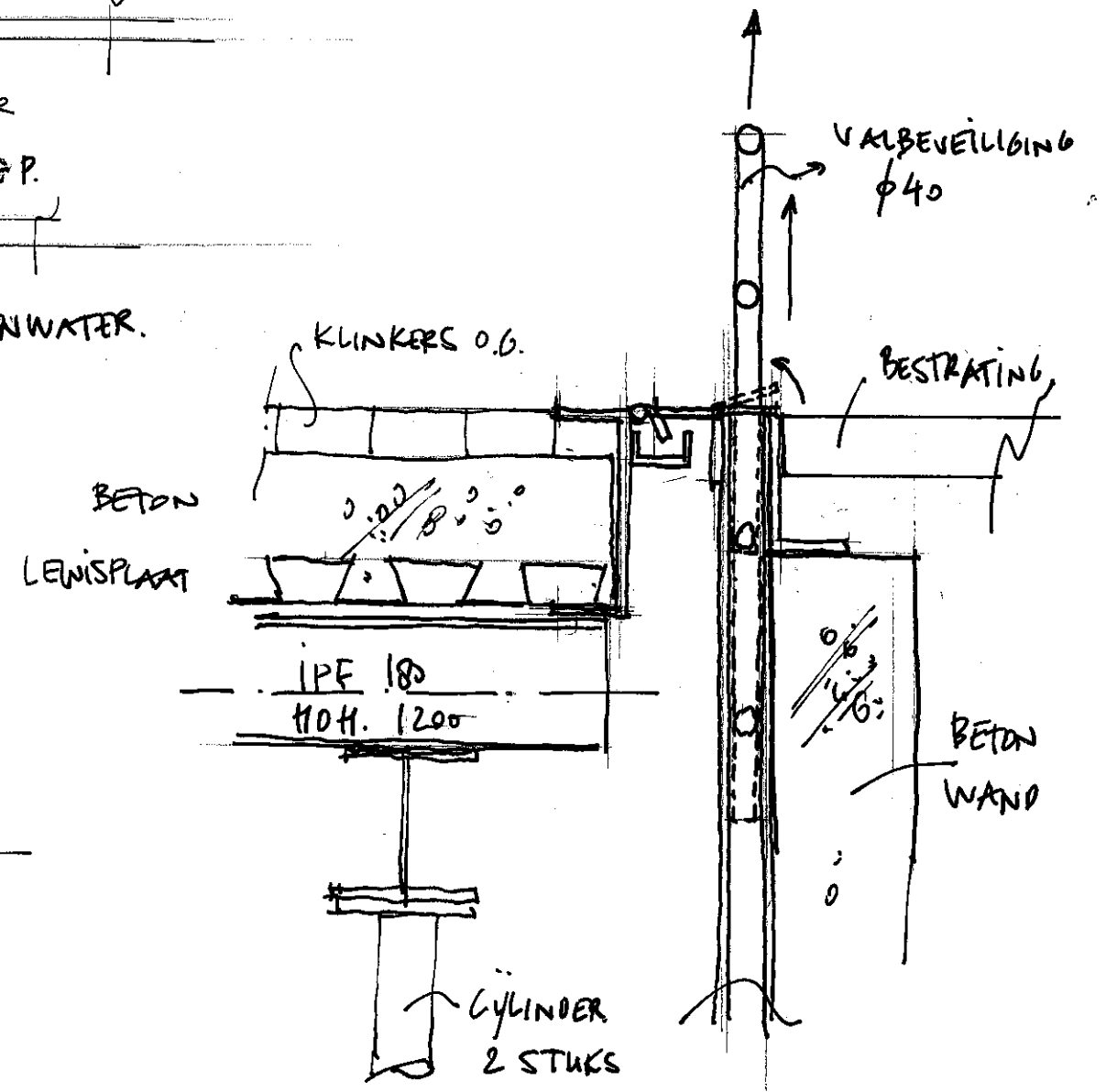
PRINCIPES DETAIL 1:10
