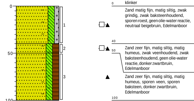
Boring: 04
