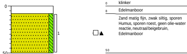
Boring: 03
