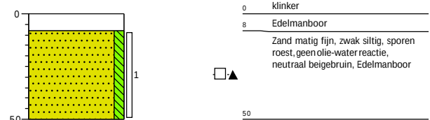
Boring: 06
