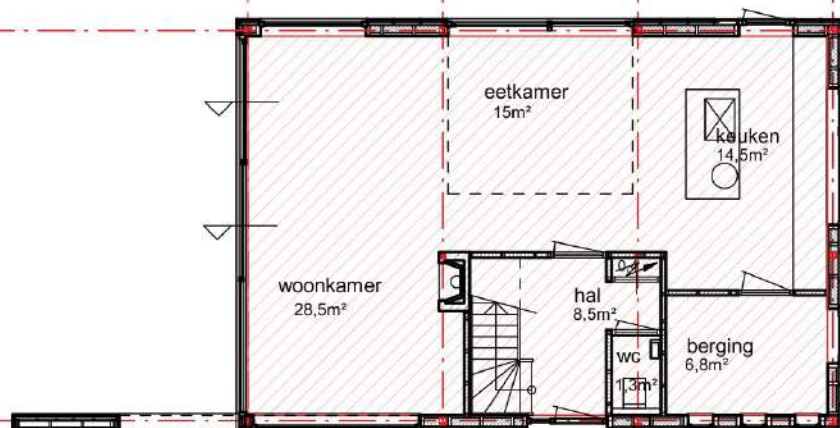
begane grond GBO = 75m²
