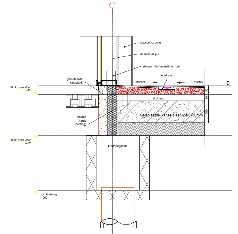
verticale details schaal 1/20
