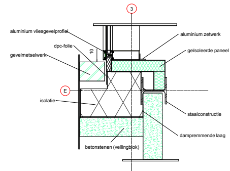
horizontale details schaal 1/20
