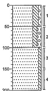
Boring: 3
