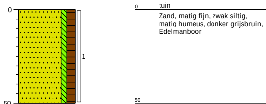
Boring: 03
