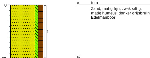
Boring: 02
