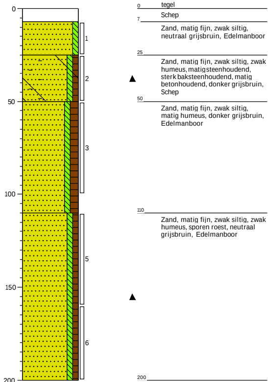
Boring: 01
