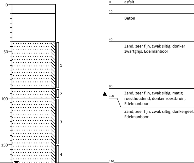
Boring: 03
