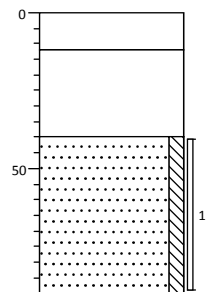
Boring: 07
