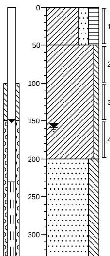
Boring: 06
