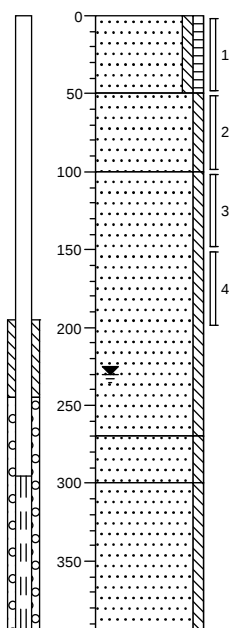
Boring: C01
