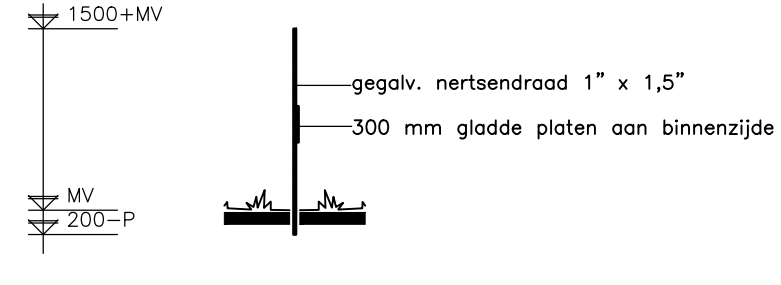
Doorsnede v.d.afrastering school 1 : 50
