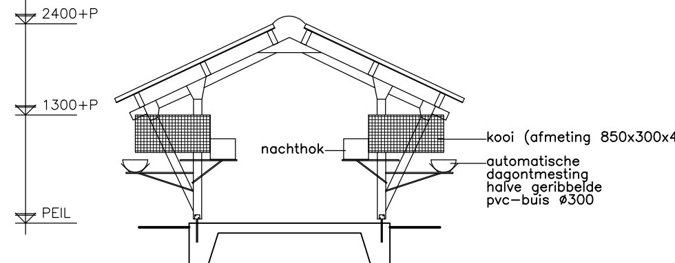
Doorsnede A-A (sheds 1 t/m 6) school 1 : 50 GL BB 94-02-013
