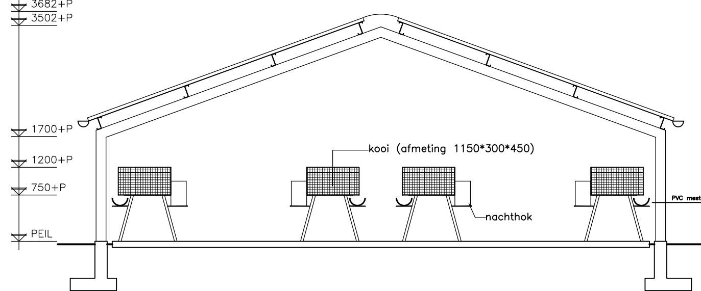
Doorsnede B-B (sheds 15 t/m 22) school 1 : 50 GL BB 94-02-013
