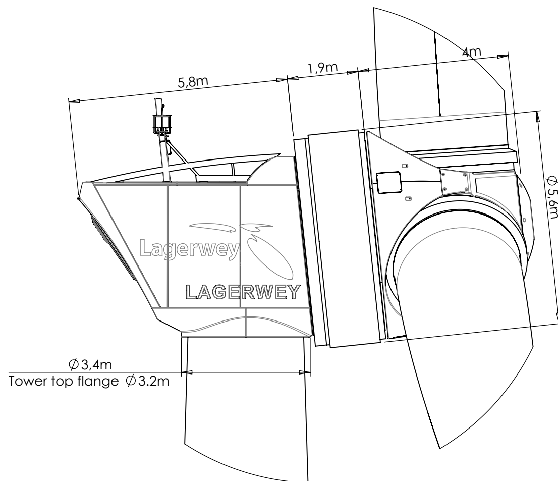
DETAIL Q
