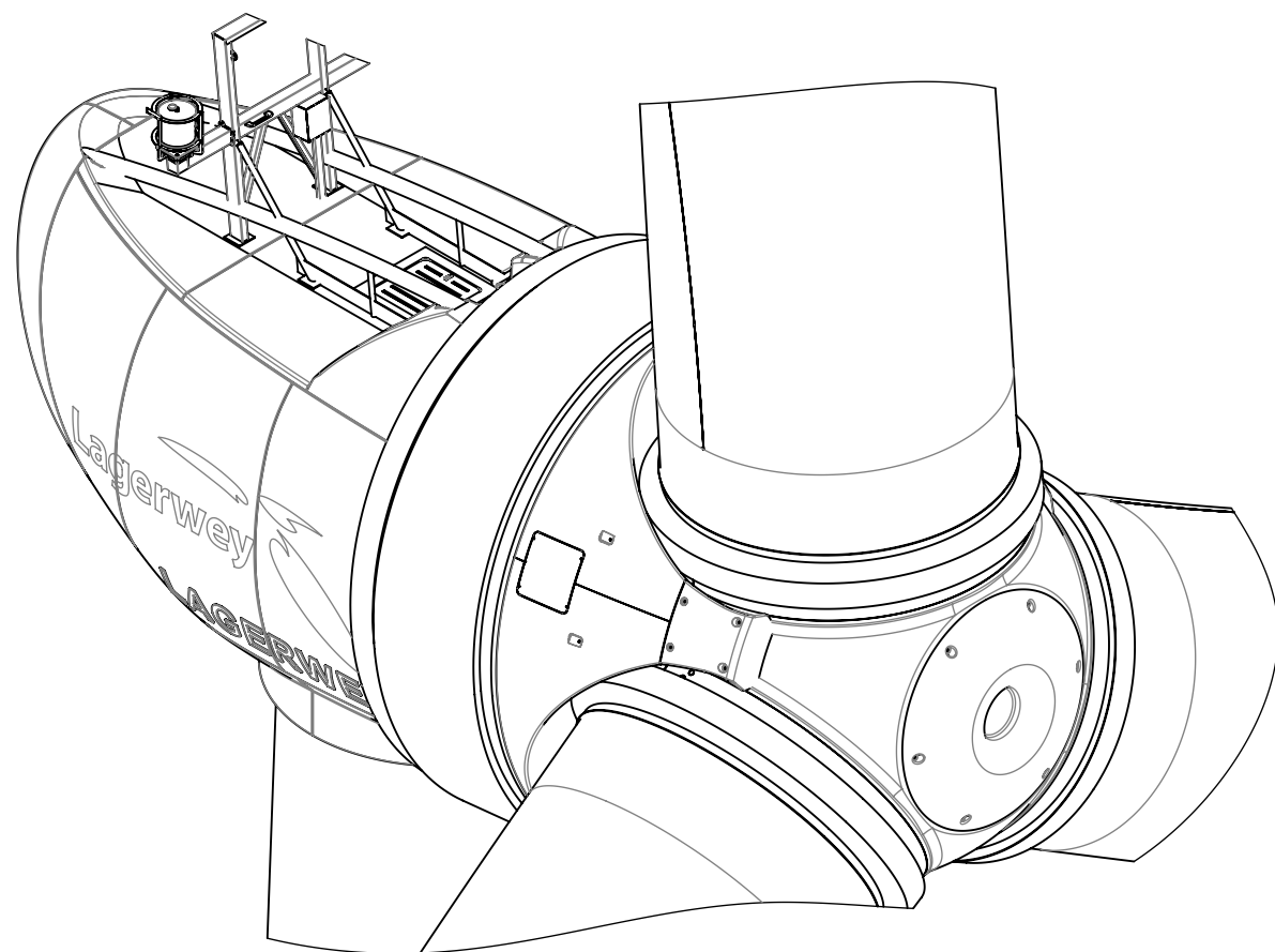
Isometric view of turbine head
